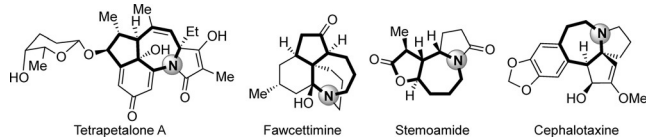
Figure 1. Natural products featuring ring-fused azepines.
